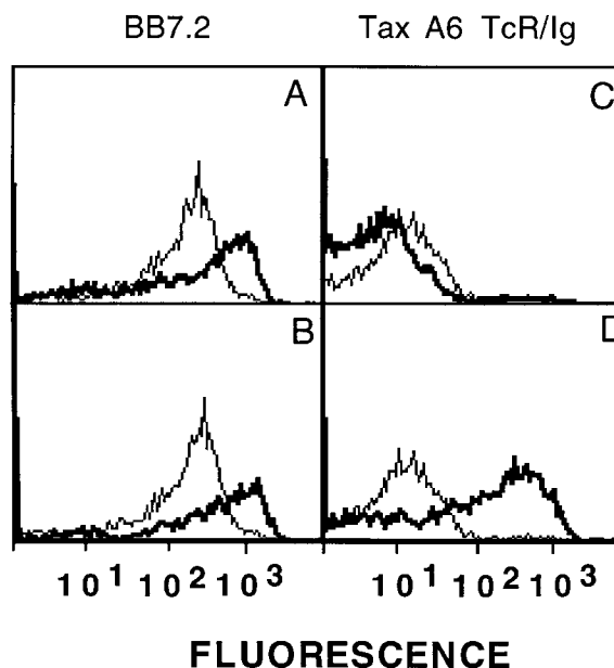
Figure 4. Divalent A6 TCR-IgG selectively reacts with HLA-A2 molecules loaded with tax 11-19 peptides. T2 cells (10 6 /ml) were incubated overnight at 37°C in the presence ( thick lines ) or absence ( thin lines ) of peptides in a 96-well plate. Cells were then pelleted and coincubated on ice with 20 μl of A6 TCR-Ig protein, with a final concentration of ~10 μg/ml, for 1 h. The peptides used in this experiment were the HLA-A2-binding peptides derived from HTLV-1 tax protein (11-19) LLFGYPVYV (B and D), and an HLA-A2-binding peptide derived from influenza M1, GILGFVFTL (A and C). Since peptides are resuspended in 50% DMSO, DMSO alone serves as a nonpeptide control. After the hour incubation with A6 TCR-Ig, cells were then washed and incubated with goat anti-mouse PE for an additional 1 h on ice, washed again, and resuspended in 250 μl of wash buffer. The experiments have been repeated at least twice. Comparable data have been obtained using either culture supernatants containing A6 TCR-Ig or purified A6 TCR-Ig. Representative histograms are shown.
